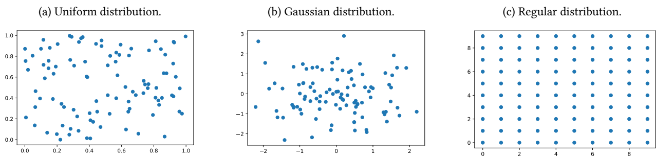
Figure 32.2: Different point patterns.
