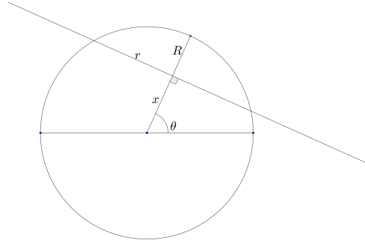
Figure 42.2: Relation between the radius of the chord and the distance to the center of the disk.
