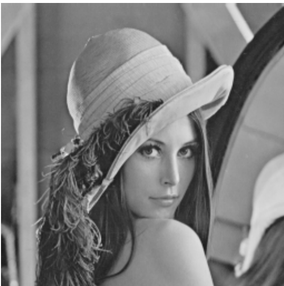
(a) lena
