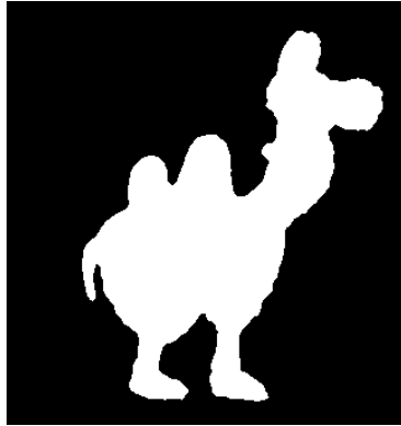
(b) Camel.
