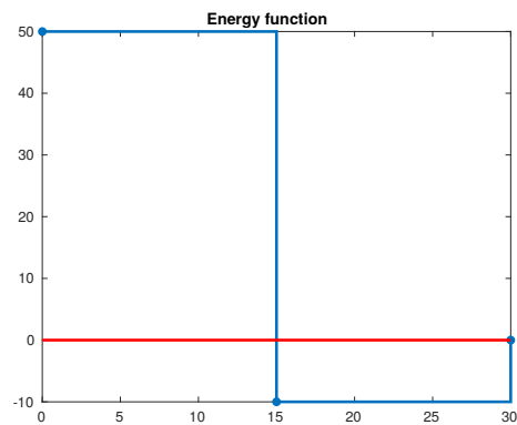
Figure 39.3: Energy function f .
