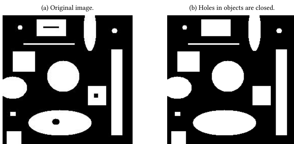
Figure 15.7: Hole filling.
