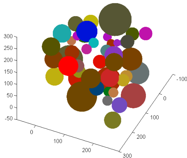
Figure 42.7: Random population of 3D overlapping spheres. This function uses povray and the vapory python API.
