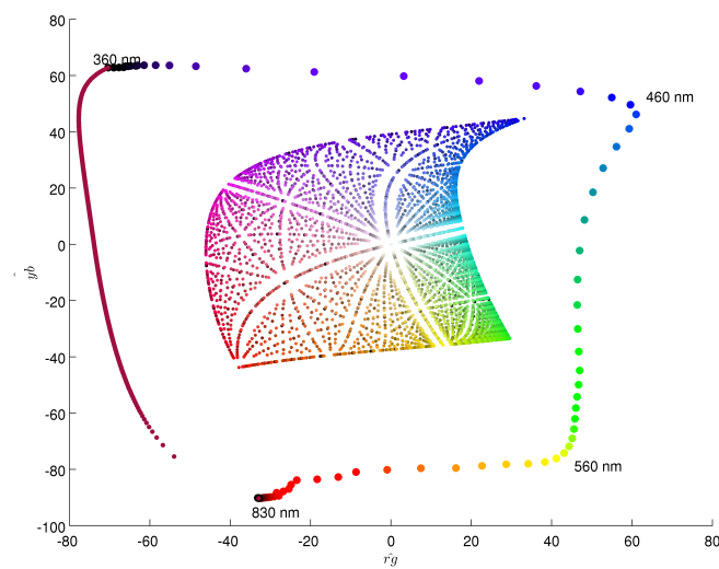
Figure 13.1: Chromaticity diagram in the plane (\hat{r}g, \hat{y}b) .
