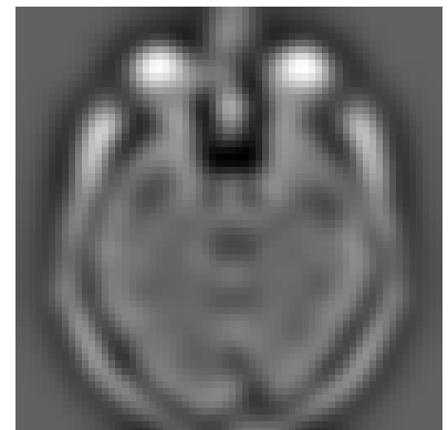
(g) Level 3.
