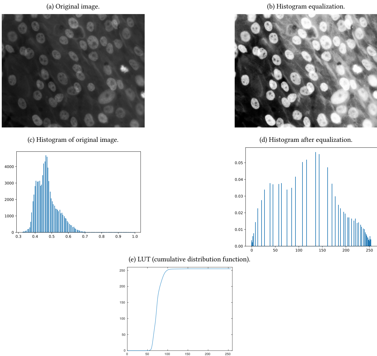
Figure 6.5: Histogram equalization.
