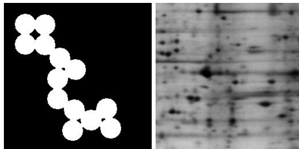
(a) circles
