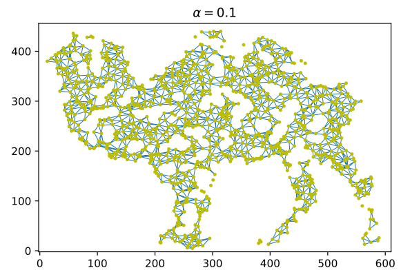
(b) \alpha = 1/10 .
