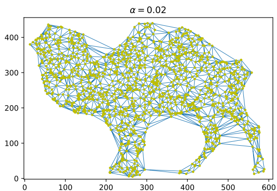
(c) \alpha = 1/50 .
