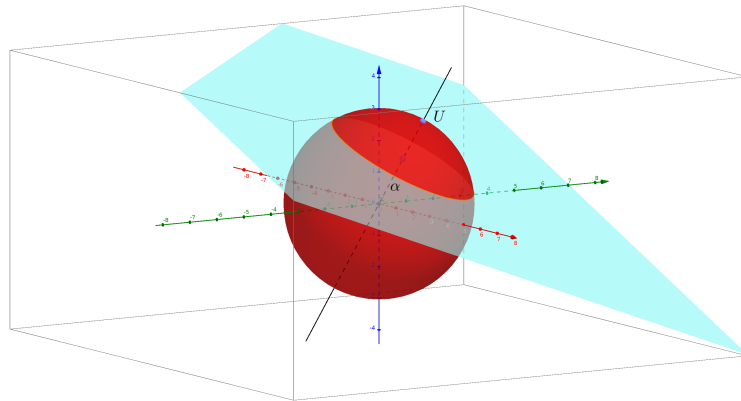
Figure 42.4: First simulation method of a random intersection of a sphere and a plane.
