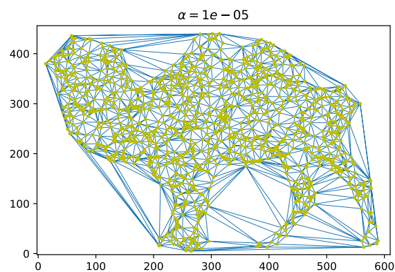
(e) \alpha = 1/100000 .
