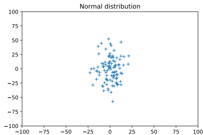
Figure 39.9: Normal distribution of points around (0, 0), with \sigma = (10, 20) .
