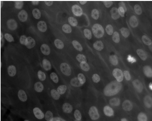
(c) E = 20 .
