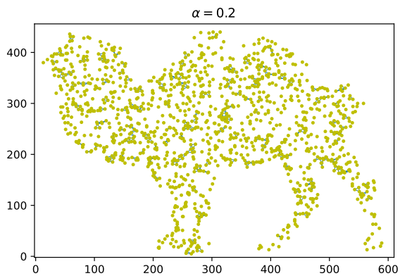
(a) \alpha = 1/5 .
