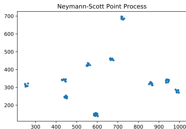
Figure 39.10: Neyman-Scott point process, with \lambda S=10 and r_{\text{Son}}=10 .
