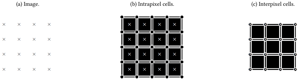
Figure 36.2: Pixels representation.
