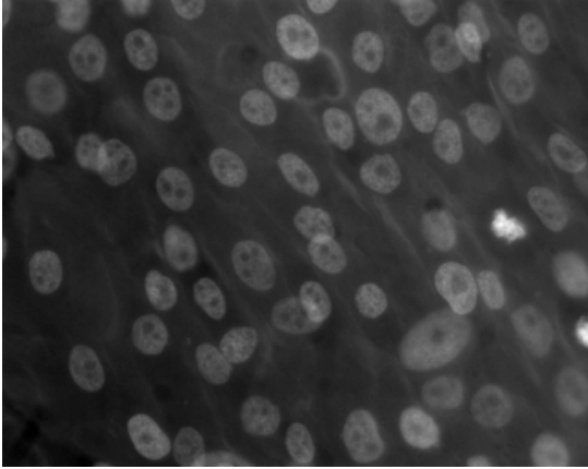
(c) \gamma = 2 .
