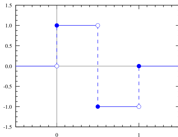
Figure 4.4: Haar wavelets. From wikipedia, author Omegatron.
