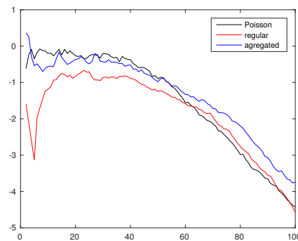
Figure 39.6: Ripley's function L(r) - r .
