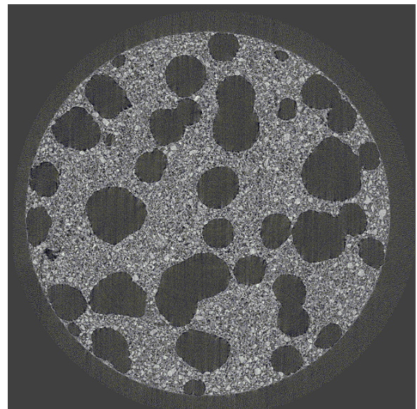
(b) cement paste (2-D section / X-ray tomography)
