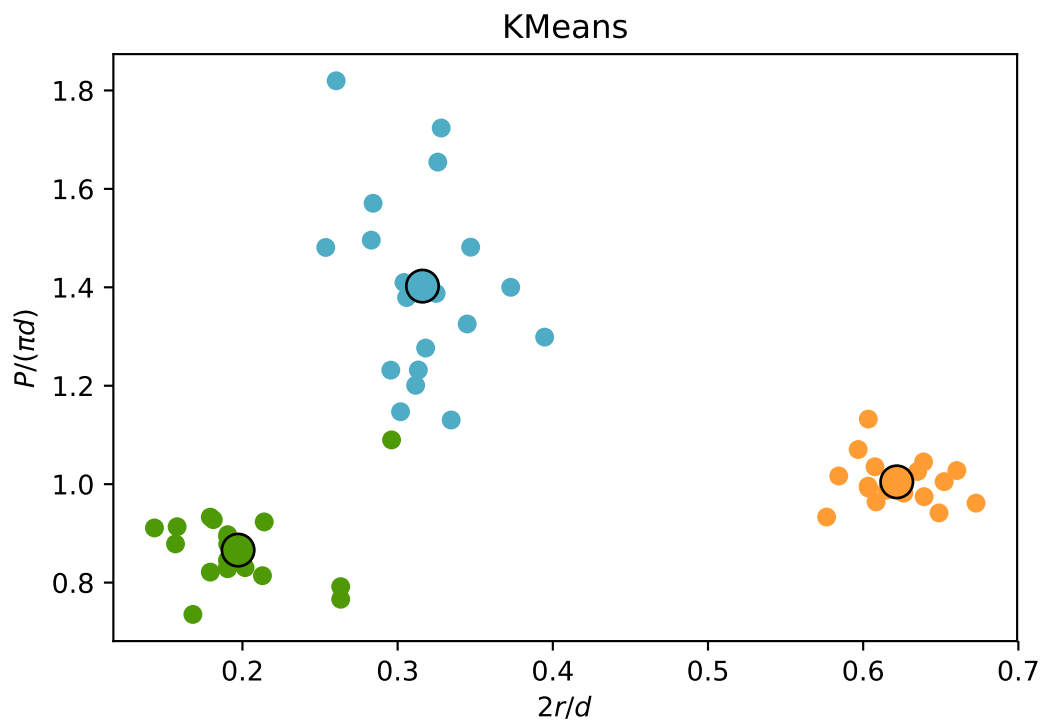
Figure 38.4: Illustration of the accuracy of the classification from a k-means method. The k-means method is not necessarily the adapted to these data. The measured accuracy if of 98.3%.
