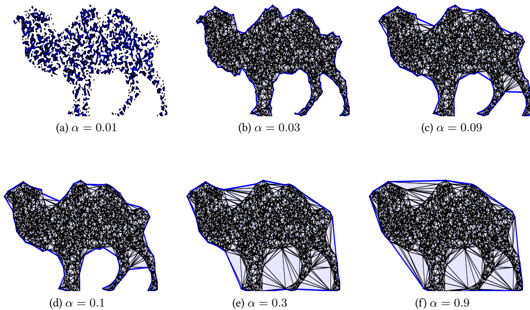
Figure 33.4: Alpha-shapes for different values of \alpha .
