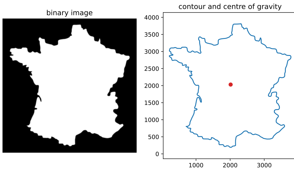
Figure 27.2: The binary image, and the contour extracted from it with its centre of gravity.
