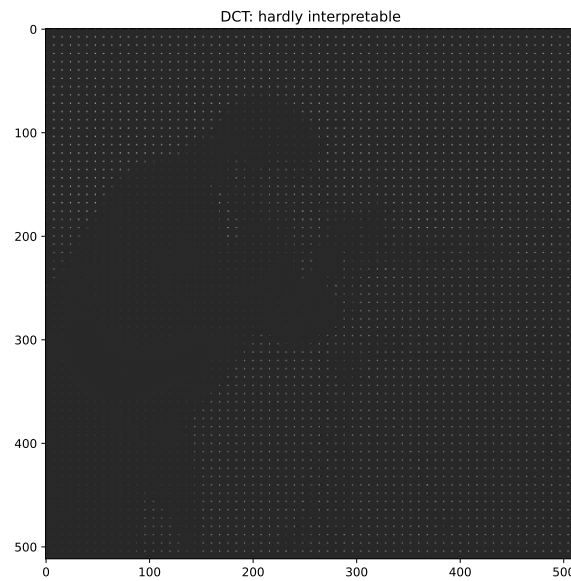
Figure 3.6: Quantized DCT coefficients of the whole image, K = 3 . Only the upper left corner of each 8 \times 8 block carries information.
