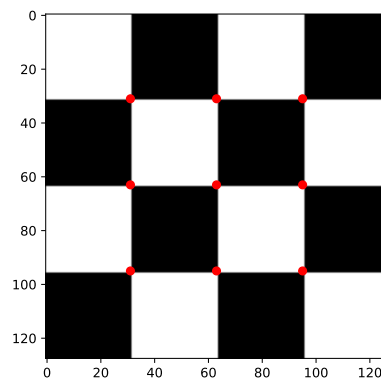
Figure 26.2: Checkerboard, and its expected corner detection.
