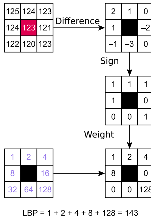
Figure 28.1: Local binary pattern. From wikipedia, author Xiawi, CC-BY-SA.
