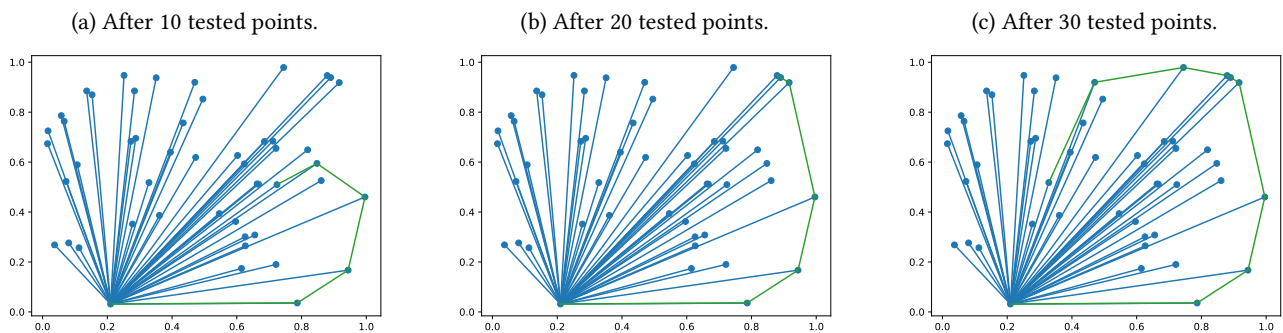
Figure 31.2: Graham scan illustration while constructing the convex hull.
