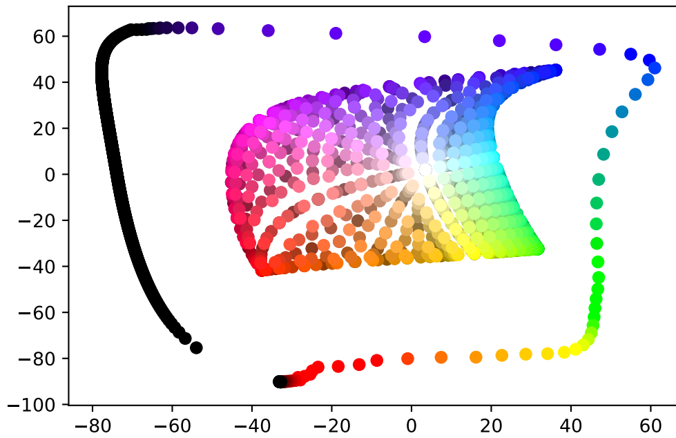
Figure 13.3: Color matching functions in the (\hat{r}g, \hat{y}b) space.
