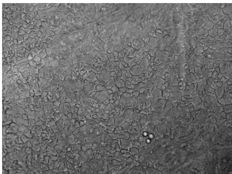
(c) Texture.
