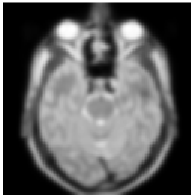
(f) Level 2.
