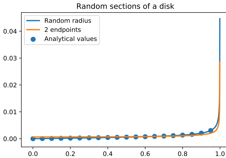
Figure 42.8: Simulations of random chords of a disk.
