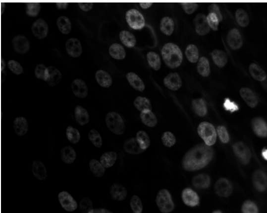
(c) \gamma = 2 .
