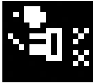
Figure 35.1: Test
