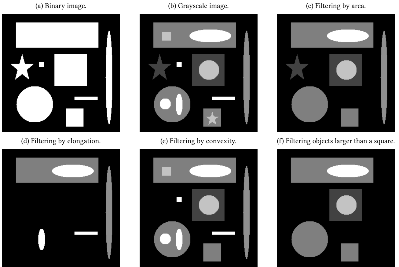
Figure 17.1: Attribute filtering examples.
