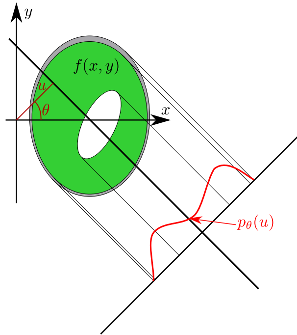
Figure 11.1: Radon transform notations.
