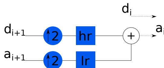
Figure 4.2: Reconstruction algorithm. The oversampling is done by inserting zeros.
