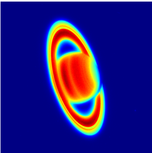
(c) Saturn.
