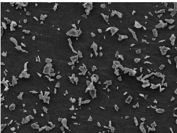
(c) Granulometry.
