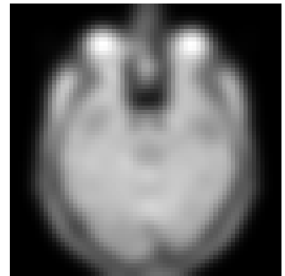
(g) Level 3.
