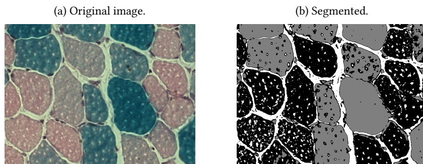
Figure 20.5: Segmentation result.
