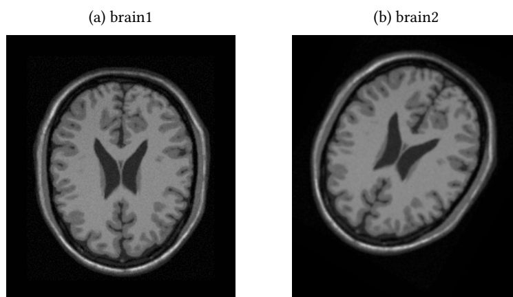
Figure 29.1: Original images.
