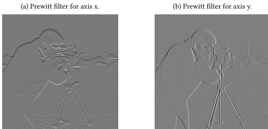
Figure 1.12: Prewitt filter.
