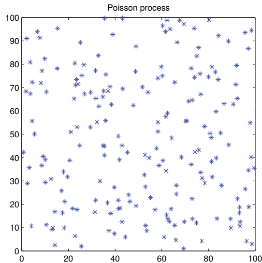
Figure 39.1: Conditional Poisson point process, with 200 points.
