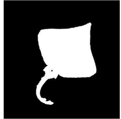
(c) Ray.
