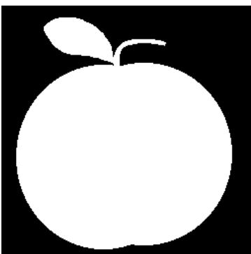
(a) Apple.
