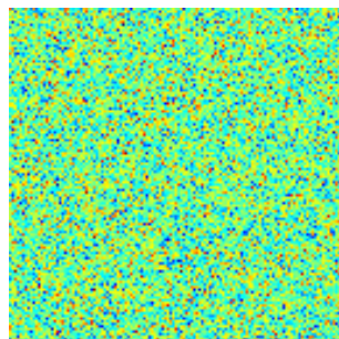
Figure 41.1: Gaussian White Noise, with m = 128 and \sigma = 30 for display purposes.
