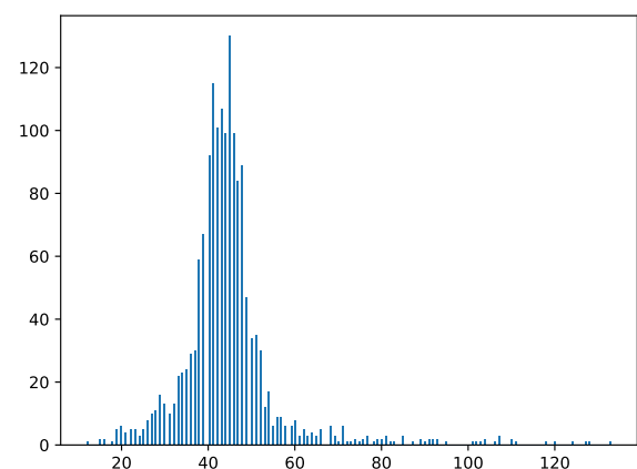
(b) Histogram.
