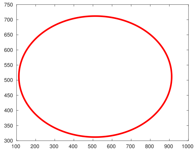
Figure 23.3: Discrete Ellipse.
