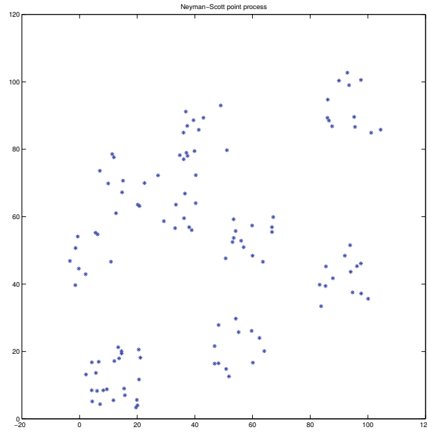
Figure 39.2: Neyman-Scott point process with h_{child} = 10 and n_{par} = 10
