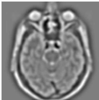
(f) Level 2.
