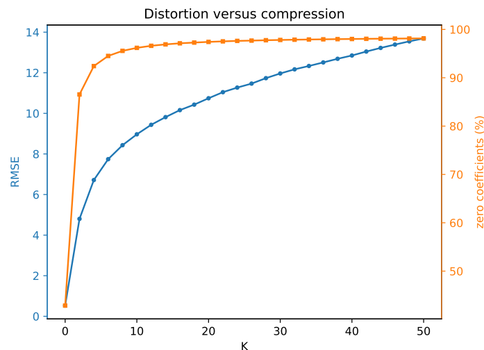
Figure 3.8: Distortion (RMSE) and proportion of zero coefficients as functions of the loss parameter K .
